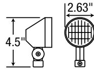
TYPE SM - PAR18 Thermoplastic
