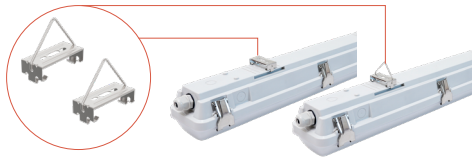
SURFACE MOUNTING AND V-HOOKS (SET OF 2)
